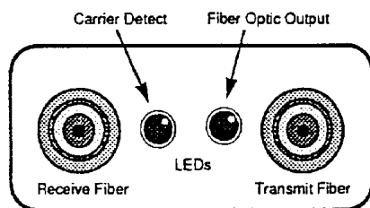
Figure 5. Back panel view of Model 1110.
