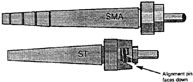
Figure 4. Close-up of ST and SMA connections.
