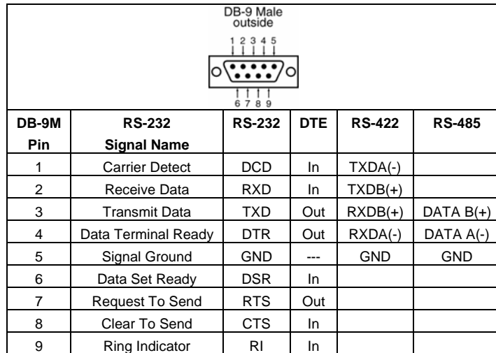
Figure 19. DB-9 Pin-outs for RS-232/422/485
