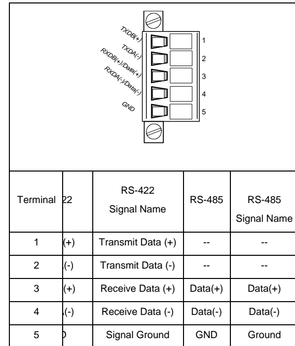
Figure 20. Terminal Block Pin-out for Vlinx ESR901W485 Serial Connection
