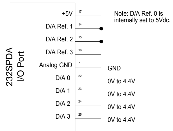
Figure 2.2 - Typical D/A Connections
