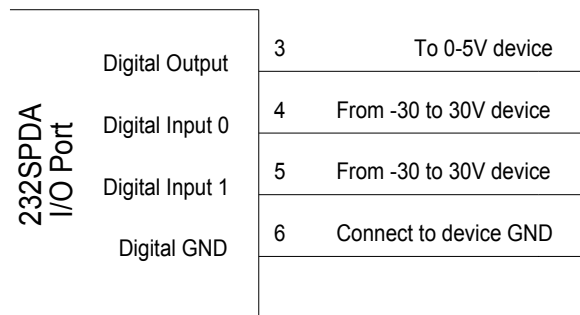
Figure 2.2 - Typical Digital I/O Connections
