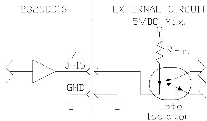
Figure 4.6 - Isolated Solid State Output
