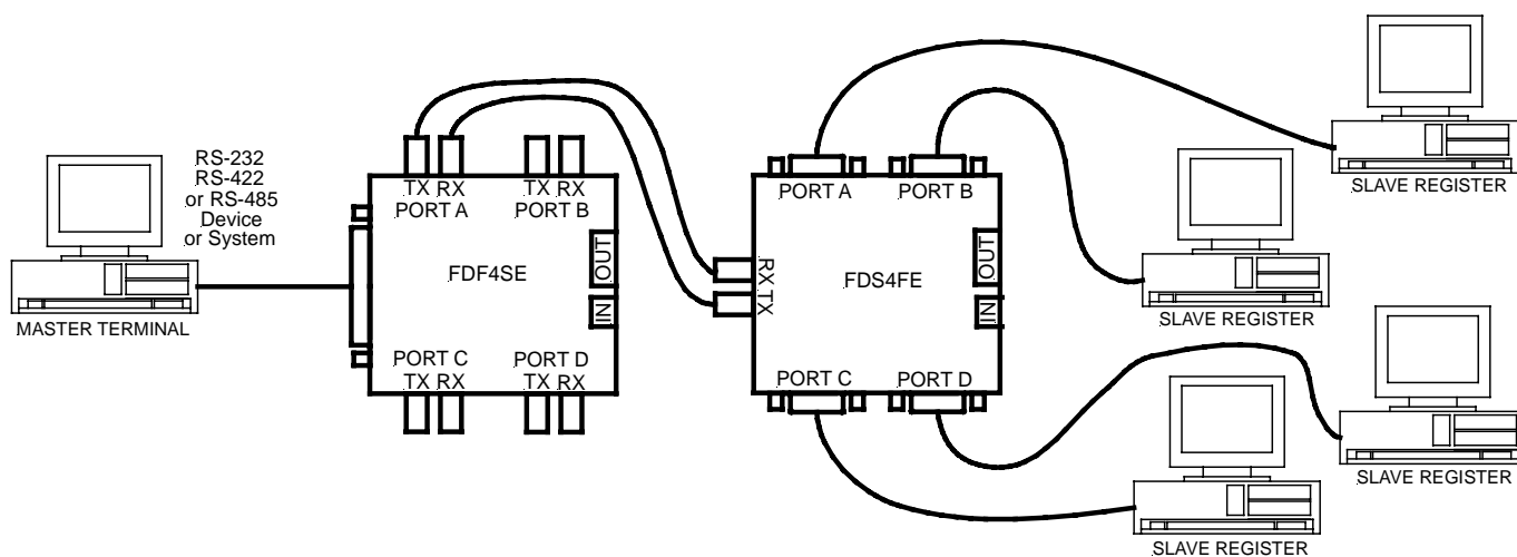
Figure 1: Typical Setup
