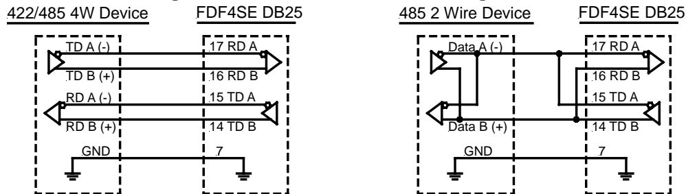
Figure 3: RS-422/485 Connection Diagrams
