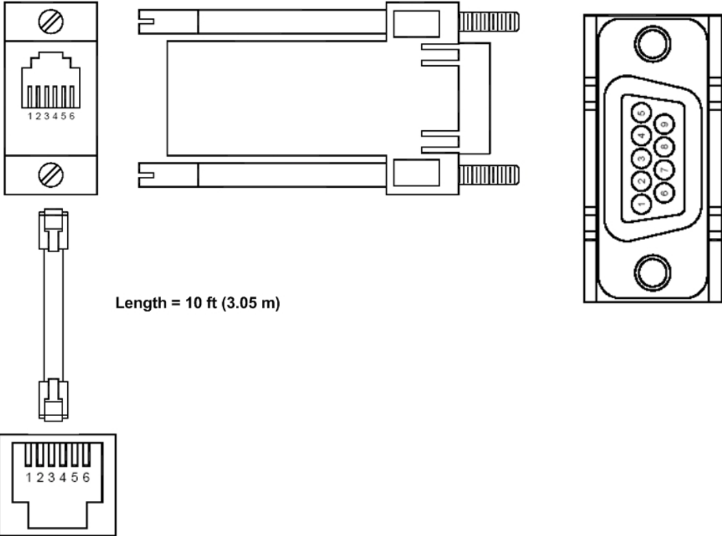
RS-232 Port from VFG
