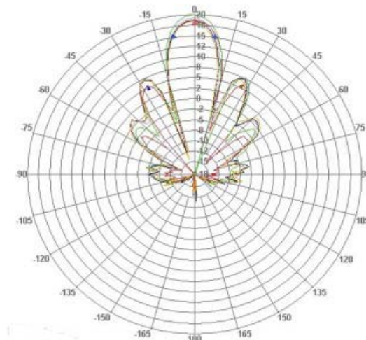
Antenna Pattern
