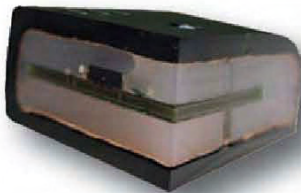
Cutaway View: 4-layer PCB in a fully shielded, impact resistant housing
